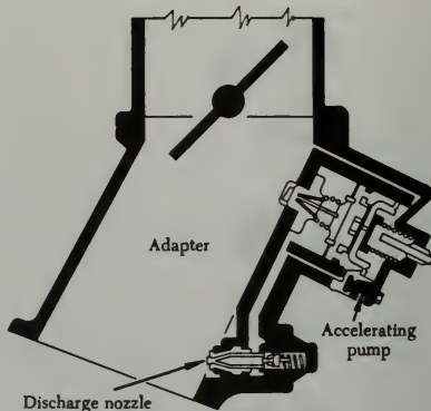
FIGURE 3-22. Adapter.
